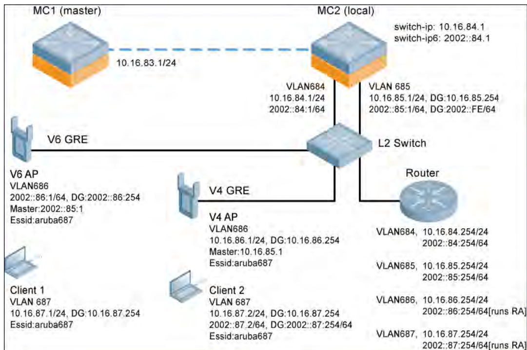
Figure 20 IPv6 Topology
