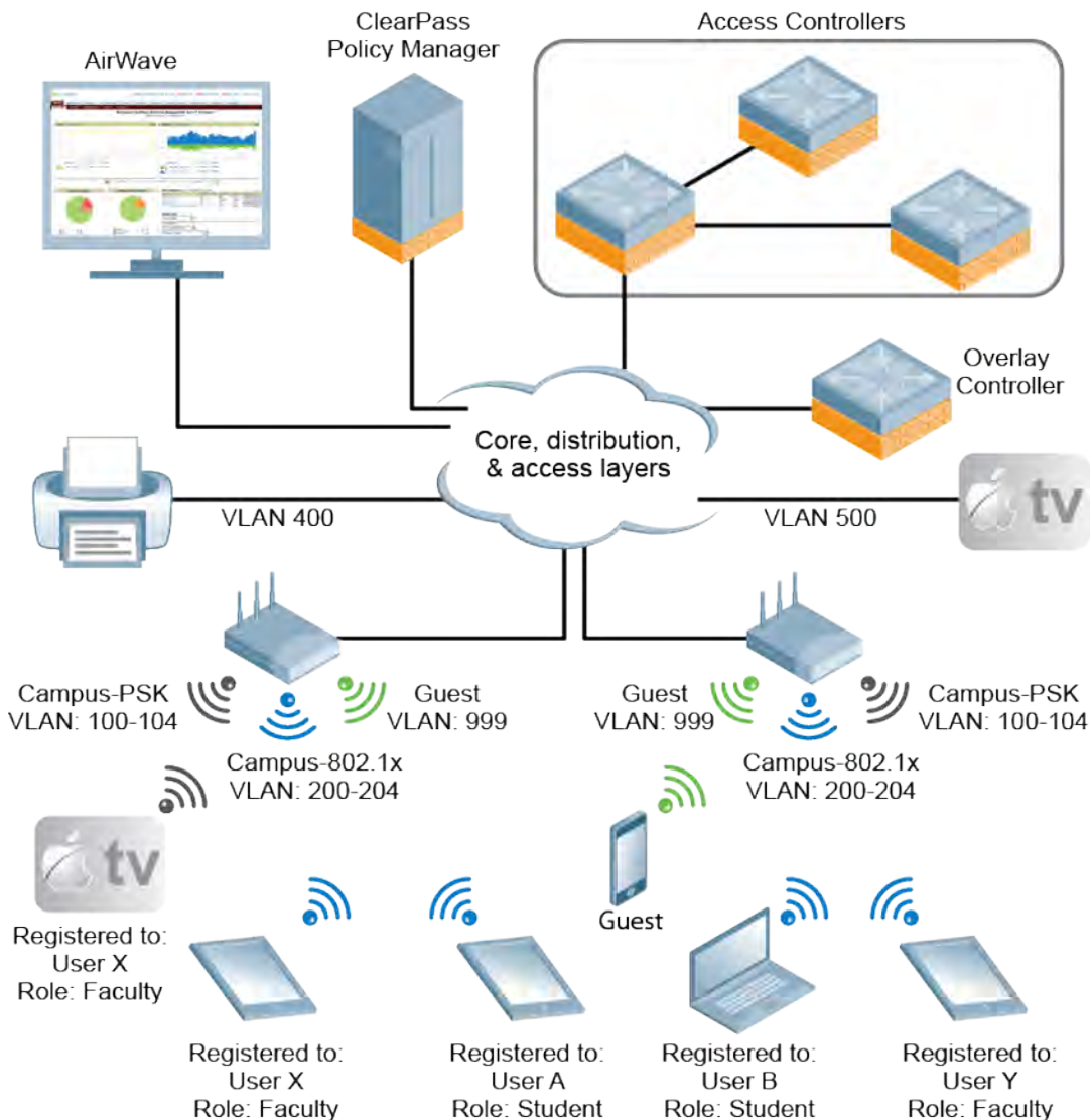
Figure 179 Overlay AirGroup Network Topology
