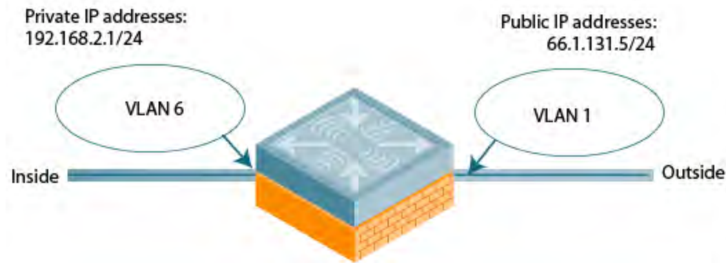
Figure 18 Example: Source NAT using Switch IP Address
