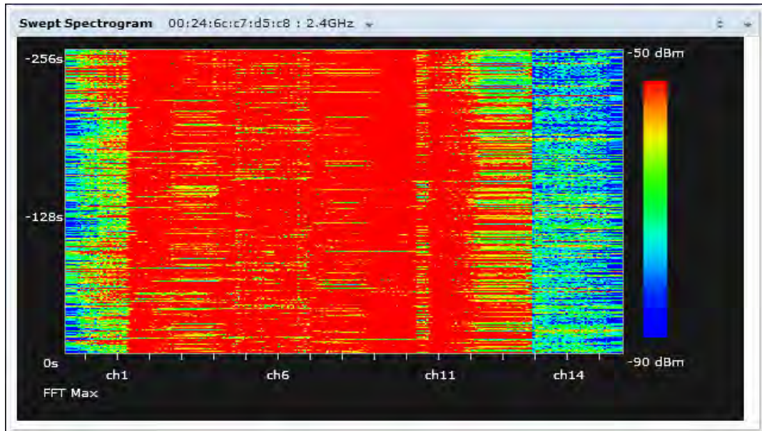
Figure 119 Swept Spectrogram
