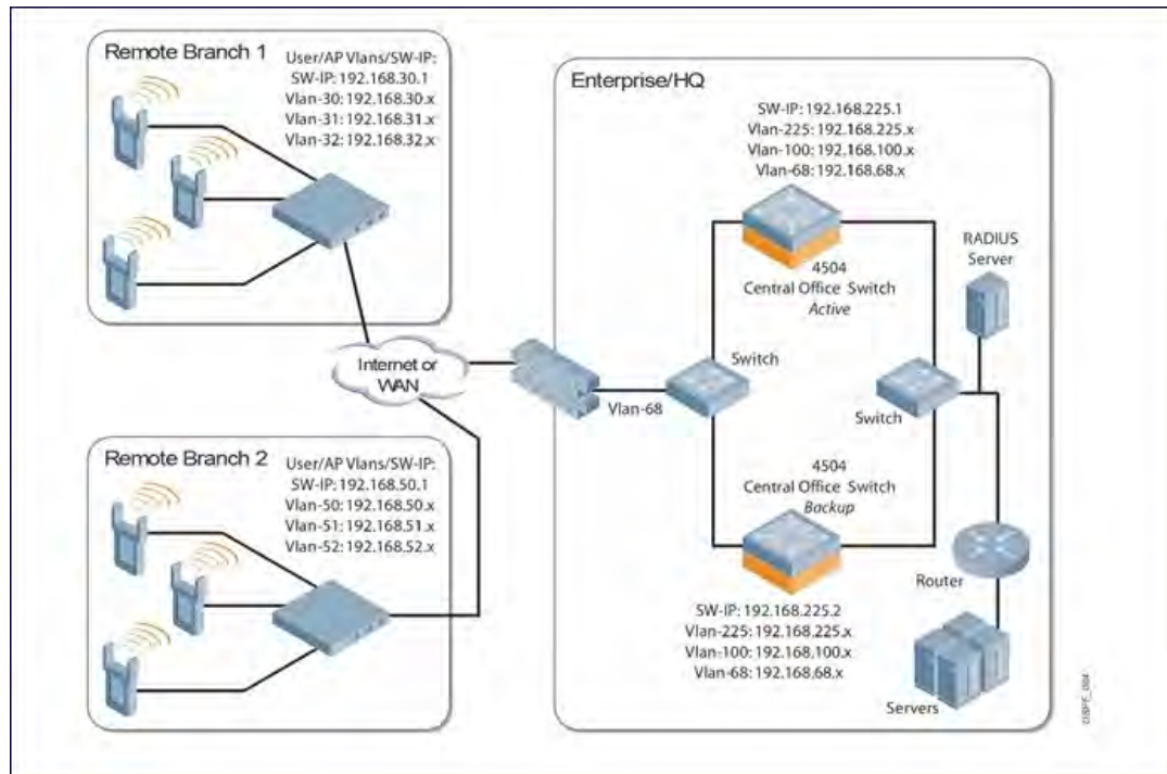
Figure 205 4306 Series Sample Topology
