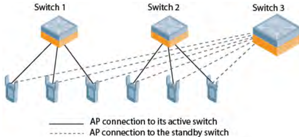
Figure 57 1:1 Active/Standby Deployment
