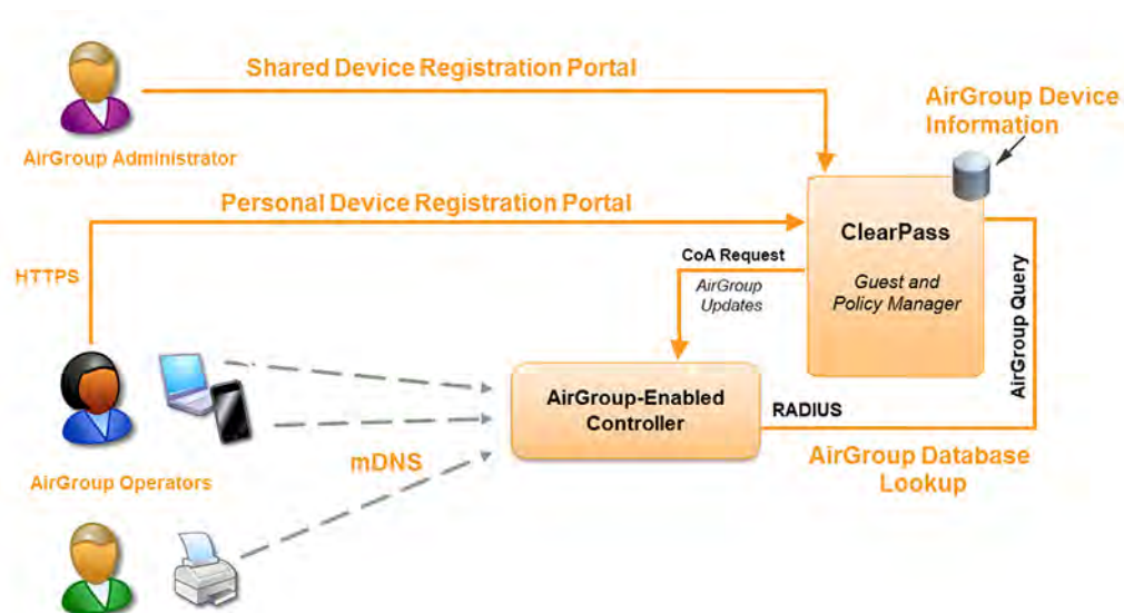
Figure 177 AirGroup in a Typical Wireless Deployment
