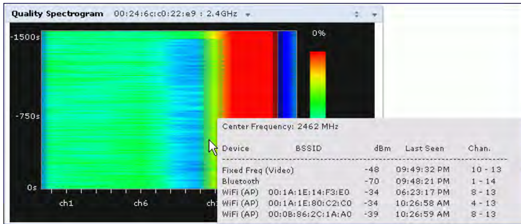
Figure 114 Quality Spectrogram
