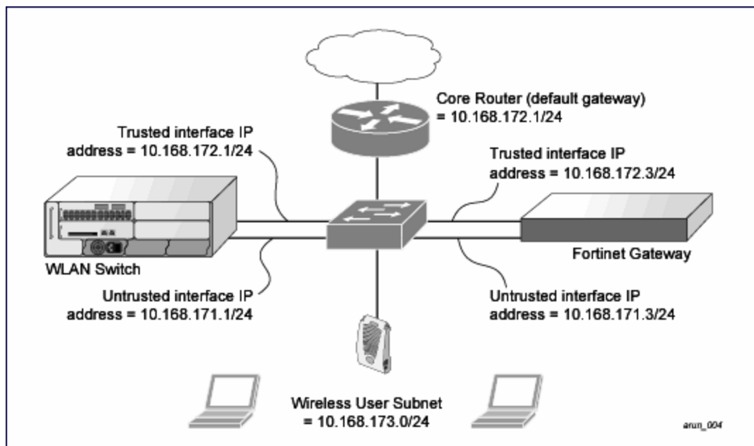
Figure 211 Example Route-Mode Topology
