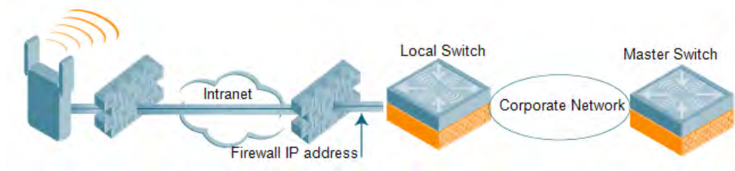
Figure 68 Remote AP in a Multi-Switch Environment
