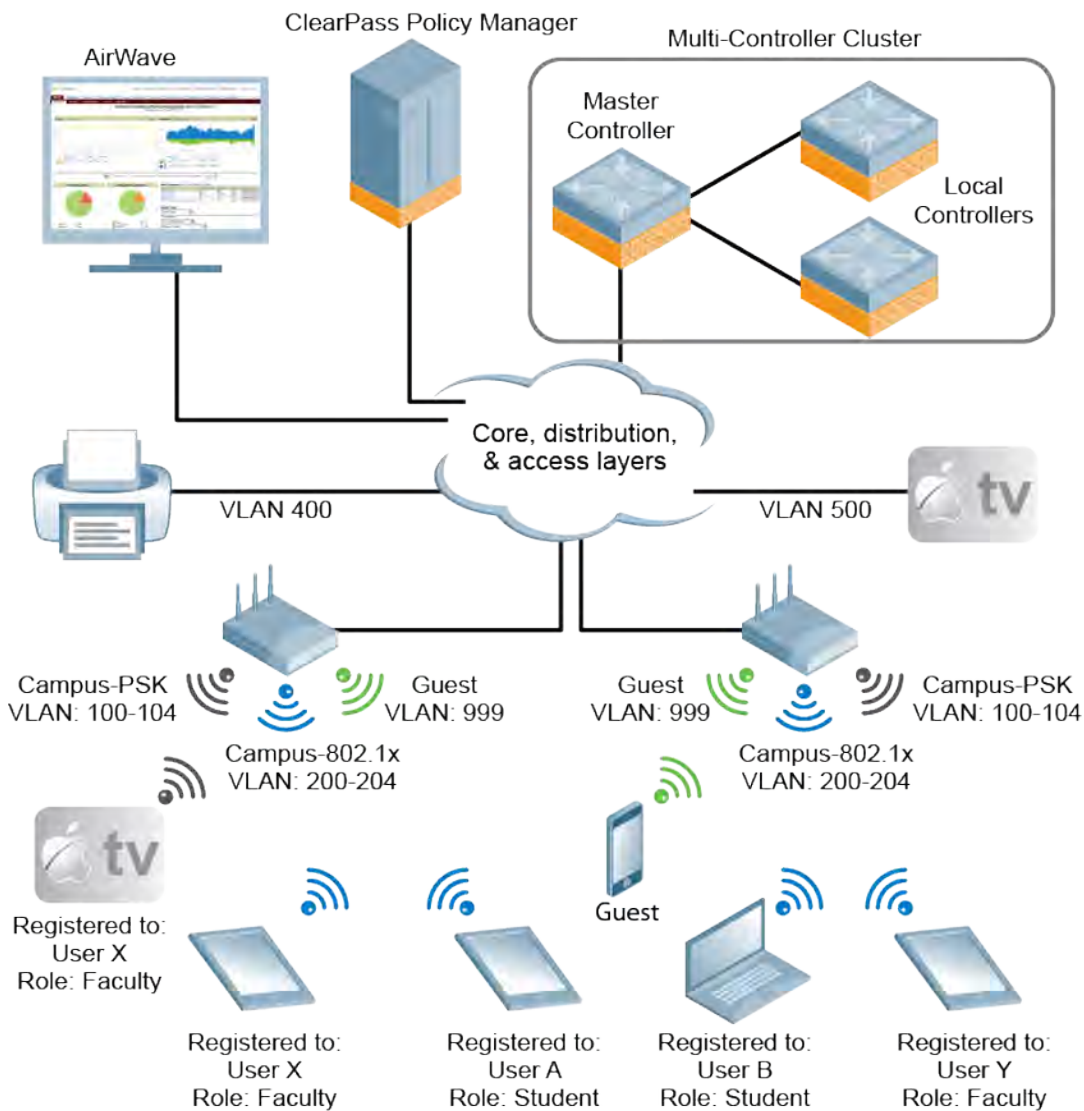
Figure 178 Integrated AirGroup Network Topology
